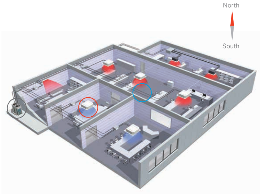
Refrigerant piping
